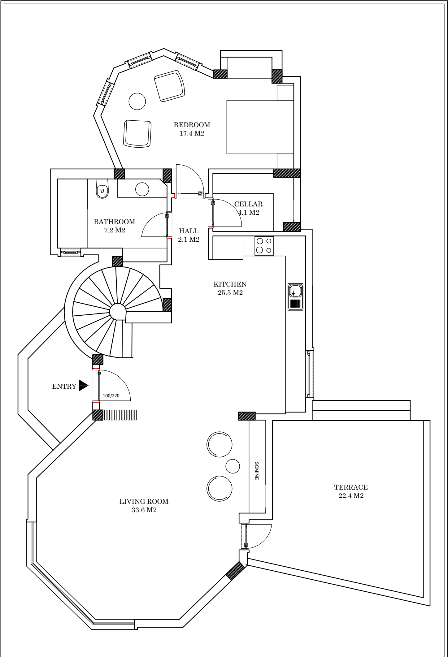
GROUND FLOOR
